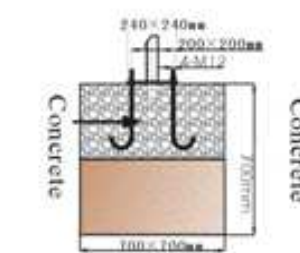
Diagram 5-1 quagginess stratum foundation drawing
