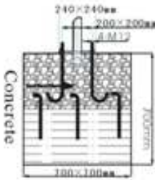
Diagram 5-2 hard rock foundation drawing
