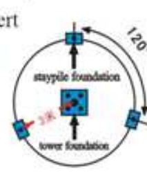
Diagram 5-4 staypile foundation diagram
